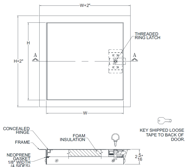
SECTION DETAIL
