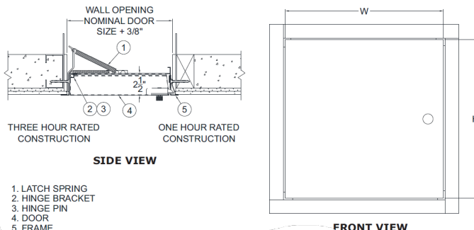
SECTION DETAIL
