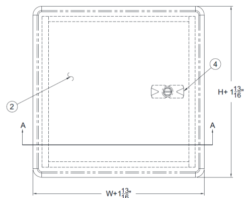
SECTION DETAIL
