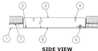
SECTION DETAIL
