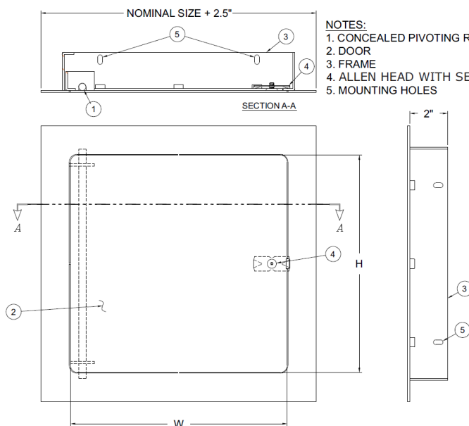
SECTION DETAIL
