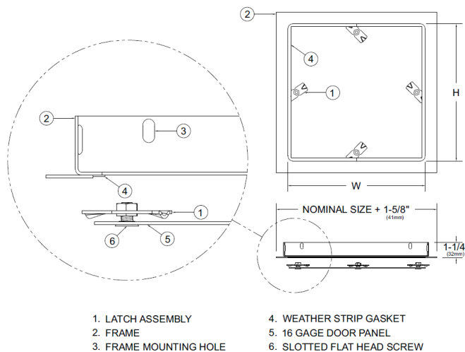
SECTION DETAIL
